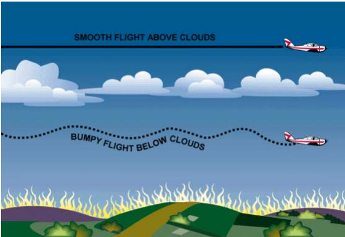
Figure 5-11.—Avoiding turbulence caused by convection currents by flying above the cloud level.
