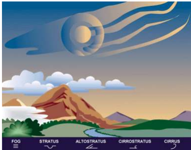
Figure 5-19.—Stratus-type clouds at various altitudes.
