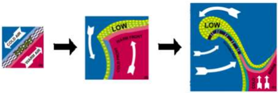
Figure 5-26.—Three stages in the development of a typical occlusion moving northeastward.
